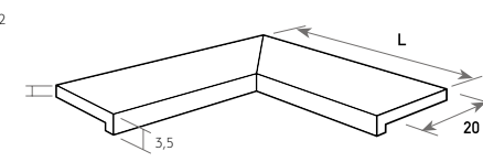
INSIDE CORNER EDGE 20xL 20x61 / 20x76 / 20x120
