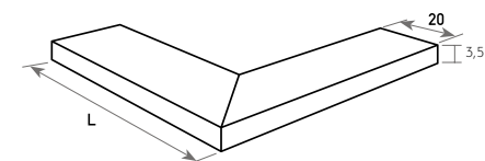
OUTSIDE CORNER EDGE 20xL 20x61 / 20x76 / 20x120
